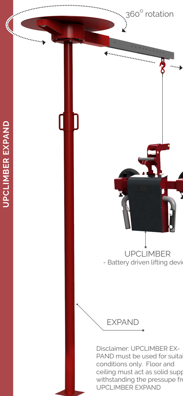
Place and assemble UPCLIMBER EXPAND on site
